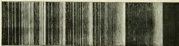
FIG. 9.—Fluting of carbon.
